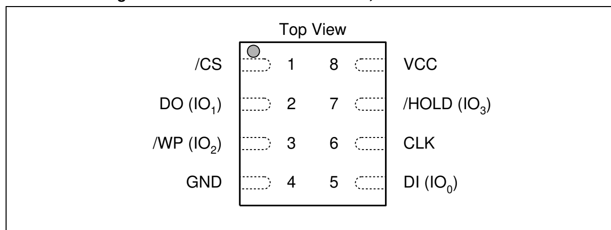
Figure 1b. W25Q64FV Pad Assignments, 8-pad WSON 6x5-mm / 8x6-mm (Package Code ZP / ZE)
